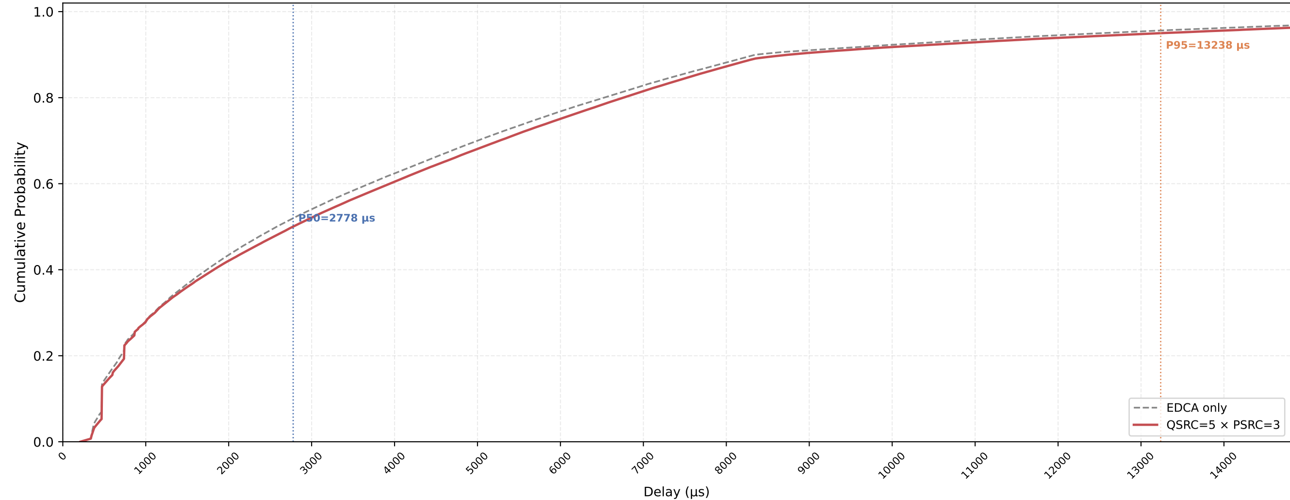
P-EDCA STA VO Delay CDF — QSRC=5 × PSRC=3 nSta=30, nPedca=30, 1Mbps, avg of 10 runs
