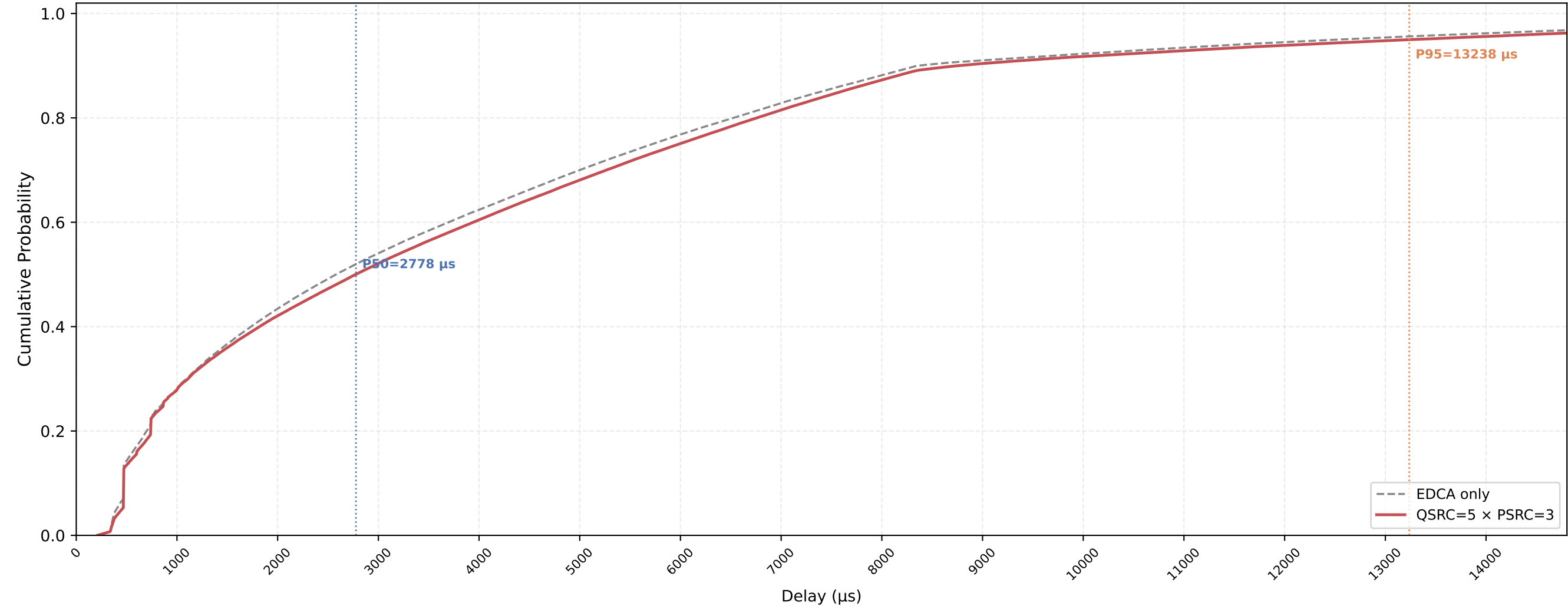
VO (all STAs) Delay CDF — QSRC=5 × PSRC=3 nSta=30, nPedca=30, 1Mbps, avg of 10 runs
