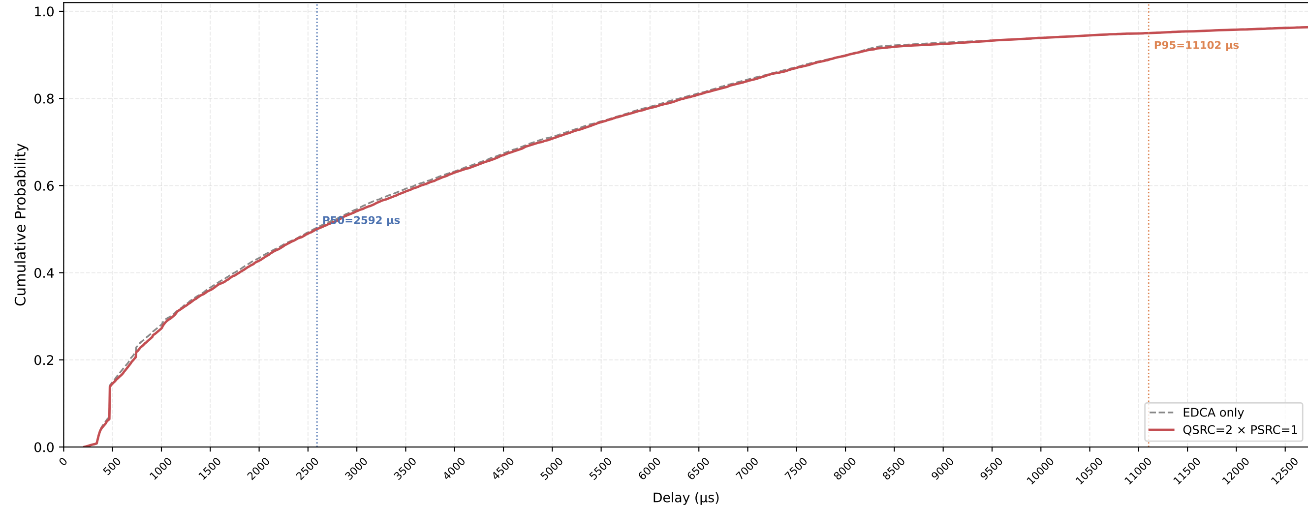
Legacy STA VO Delay CDF — QSRC=2 × PSRC=1 nSta=30, nPedca=5, 1Mbps
