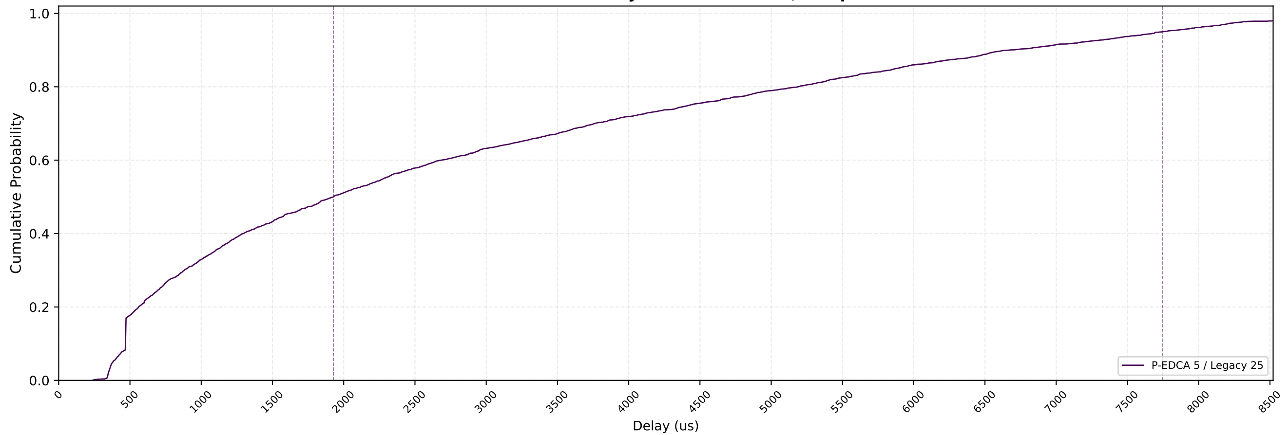
P-EDCA STAs Delay CDF — nSta=30, 1Mbps
