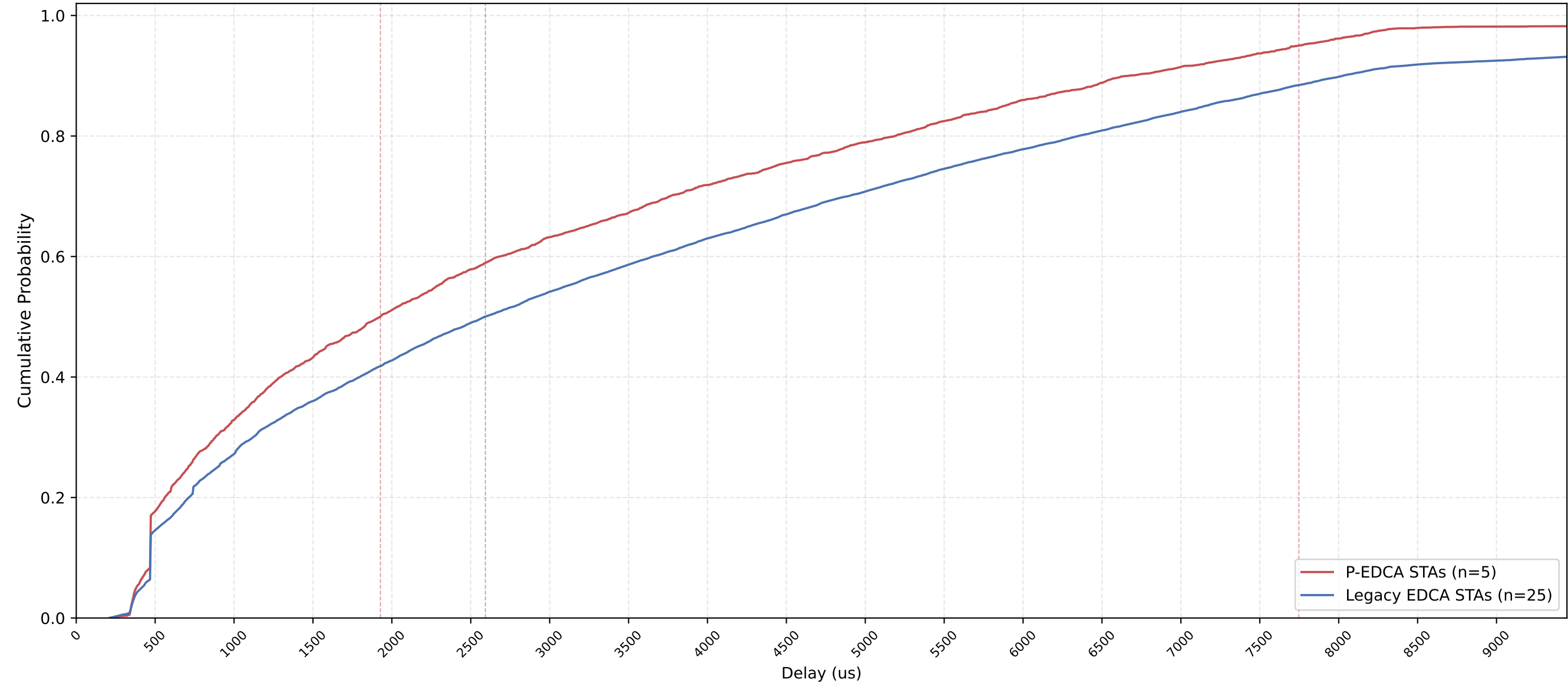
P-EDCA vs Legacy Delay CDF — n_pedca=5, n_legacy=25, nSta=30, 1Mbps
