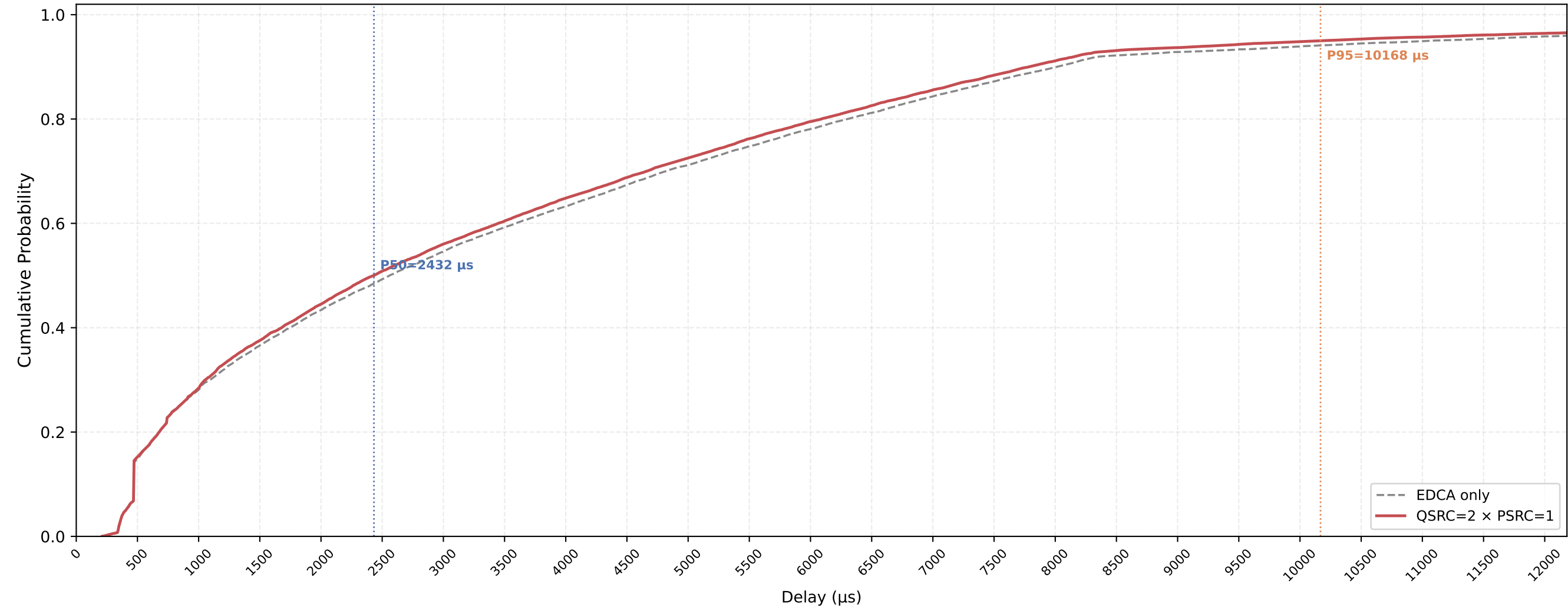
VO (all STAs) Delay CDF — QSRC=2 × PSRC=1 nSta=30, nPedca=5, 1Mbps
