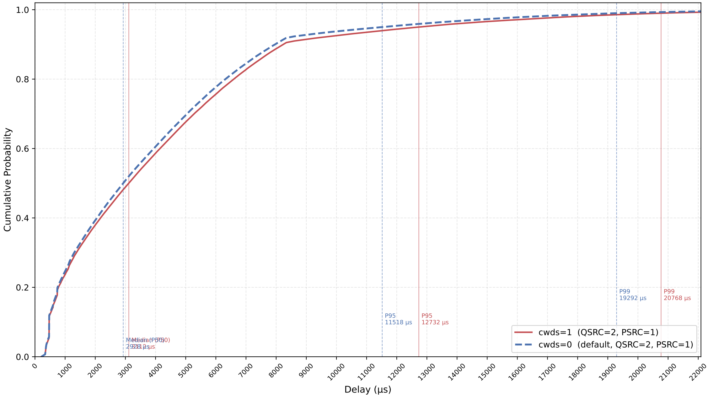
VO Delay CDF: cwds=0 vs cwds=1 — nSta=30, nPedca=15, QSRC=2, PSRC=1, 1Mbps, avg of 10 runs
