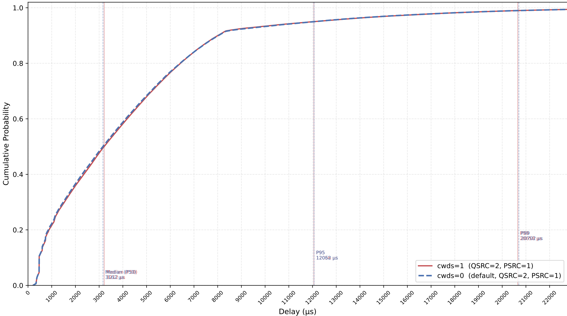
VO Delay CDF: cwds=0 vs cwds=1 — nSta=30, nPedca=30, QSRC=2, PSRC=1, 1Mbps, avg of 10 runs
