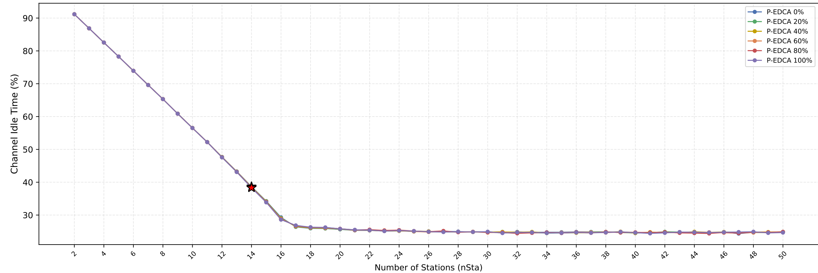
Channel Idle Time vs nSta — (Red Star = Current nSta=14)
