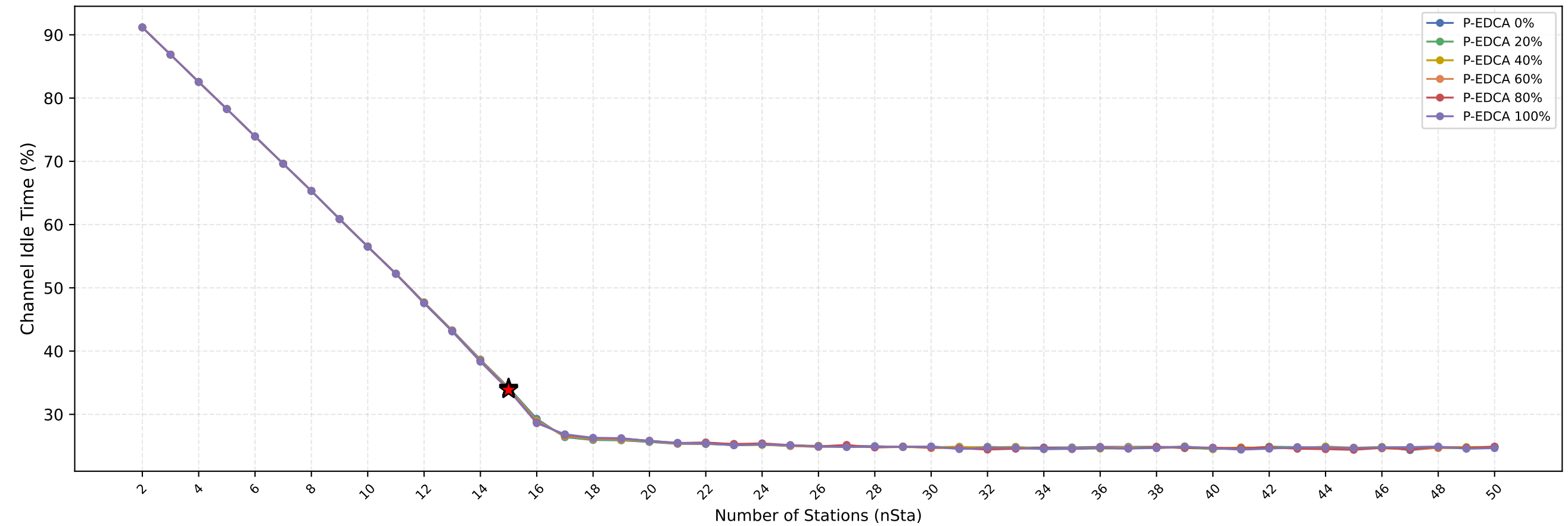
Channel Idle Time vs nSta — (Red Star = Current nSta=15)
