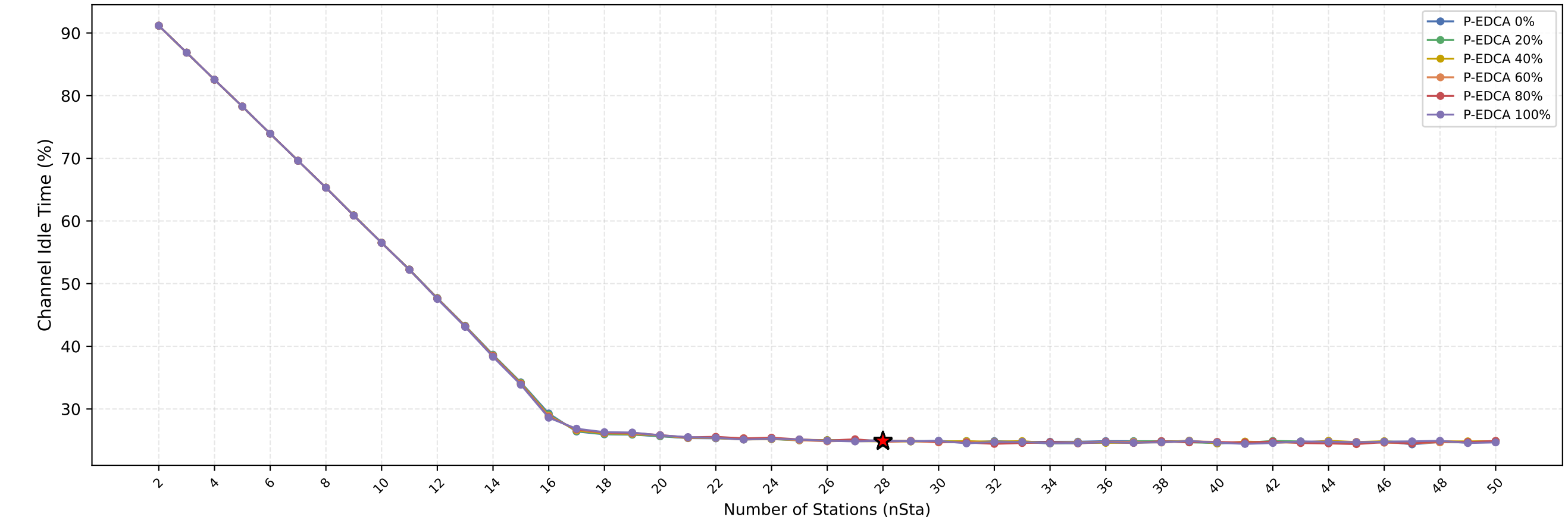
Channel Idle Time vs nSta — (Red Star = Current nSta=28)
