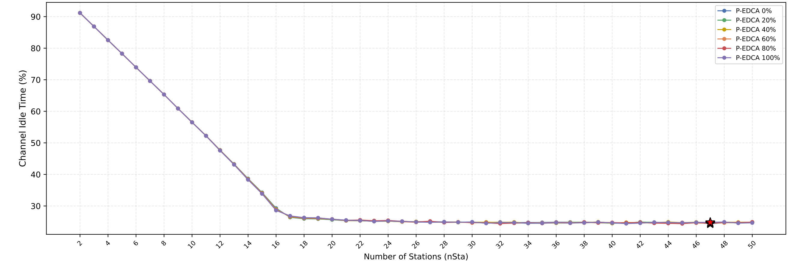
Channel Idle Time vs nSta — (Red Star = Current nSta=47)
