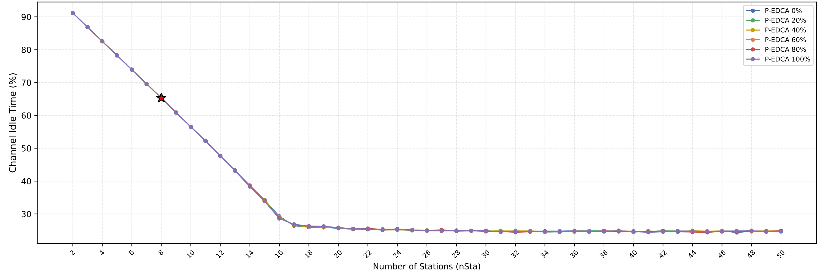
Channel Idle Time vs nSta — (Red Star = Current nSta=8)
