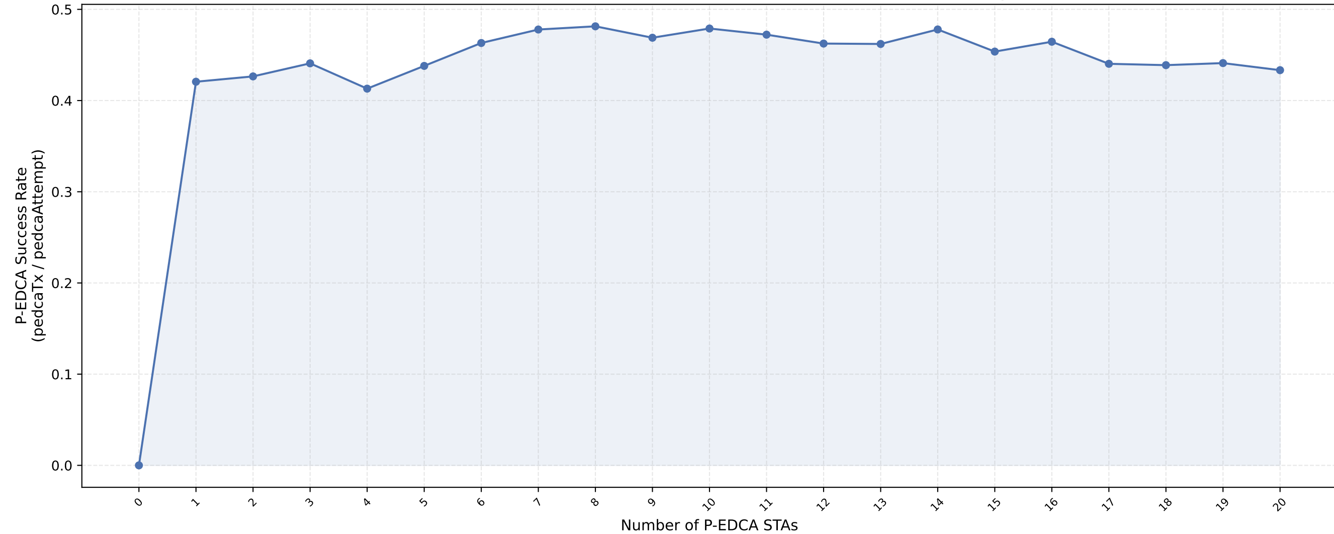
P-EDCA Success Rate: \text{pedcaTx} / \text{pedcaAttempt} — nSta=20, 1Mbps (avg of 10 runs)
