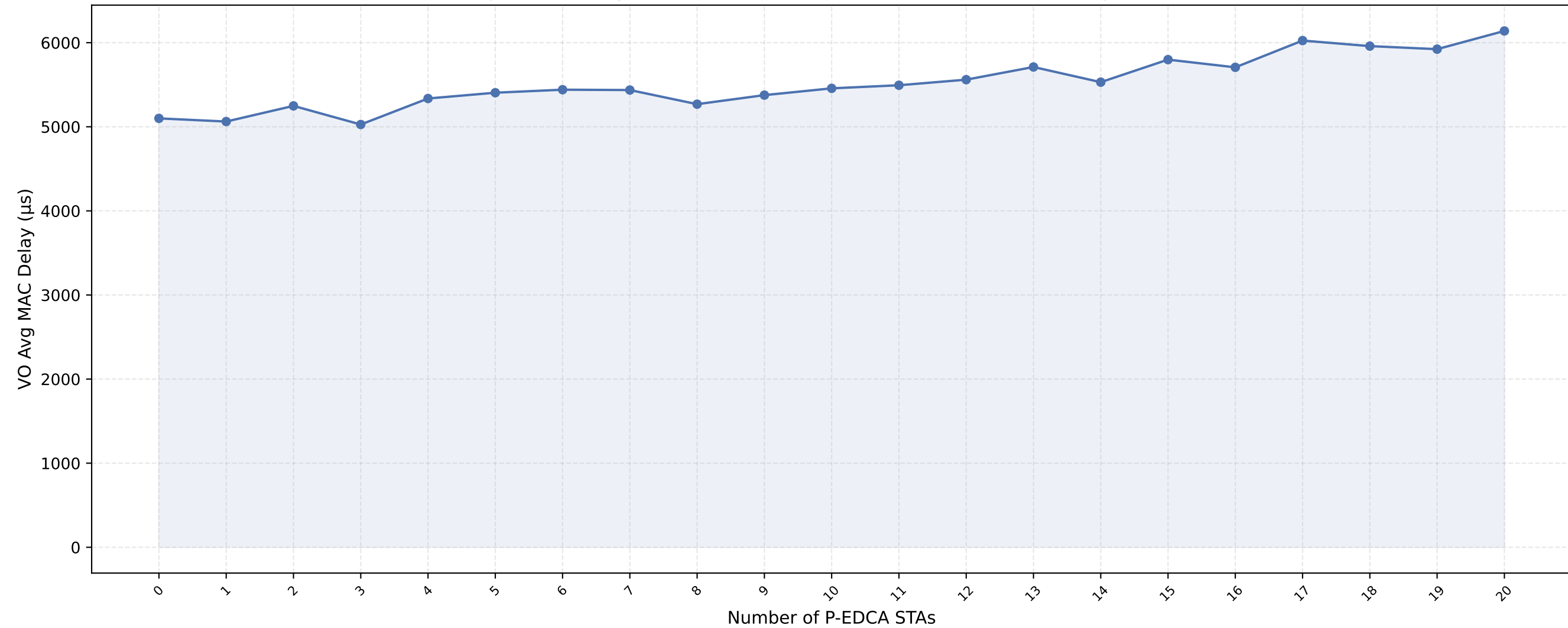
VO Avg MAC Delay vs P-EDCA STAs — nSta=20, 1Mbps (avg of 10 runs)
