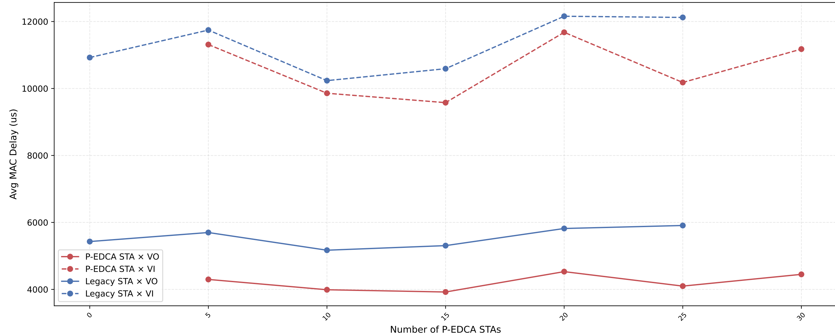
P-EDCA vs Legacy x VO/VI Avg MAC Delay - nSta=30, 1Mbps (avg of 10 runs)
