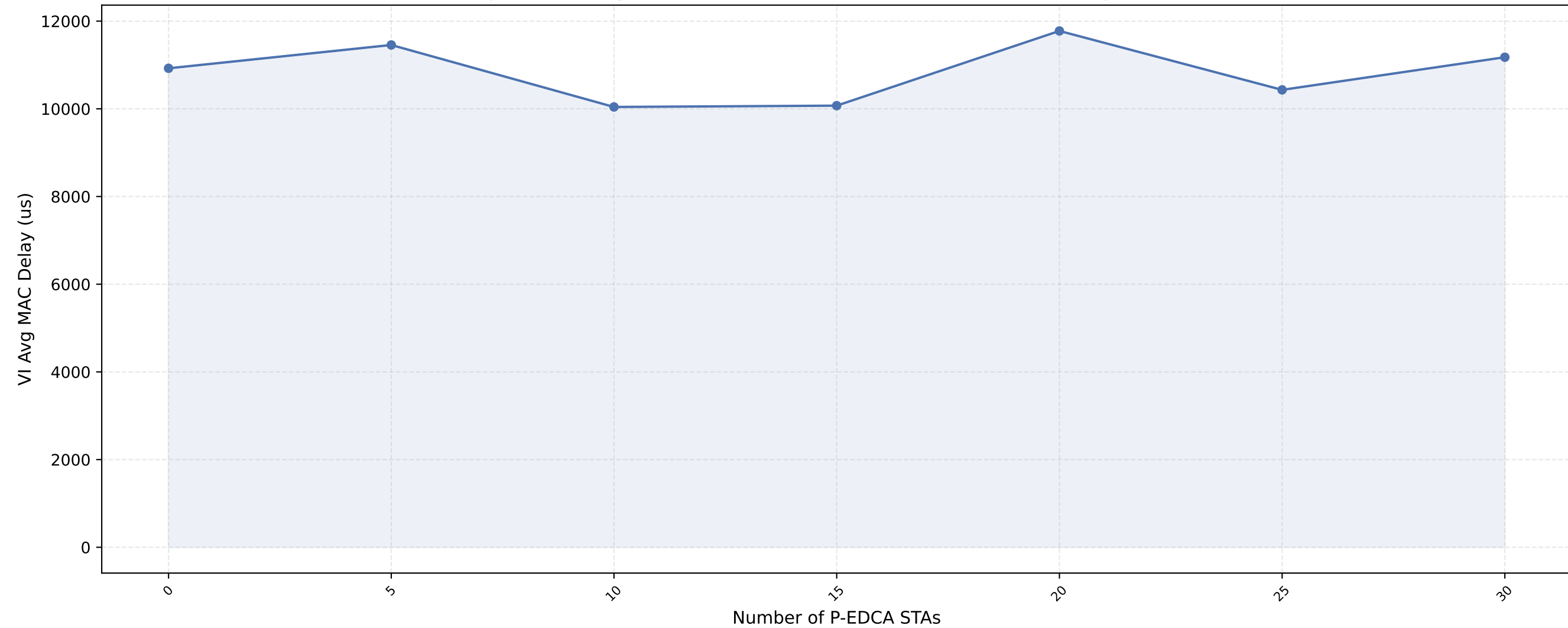
VI Avg MAC Delay vs P-EDCA STAs — nSta=30, 1Mbps (avg of 10 runs)
