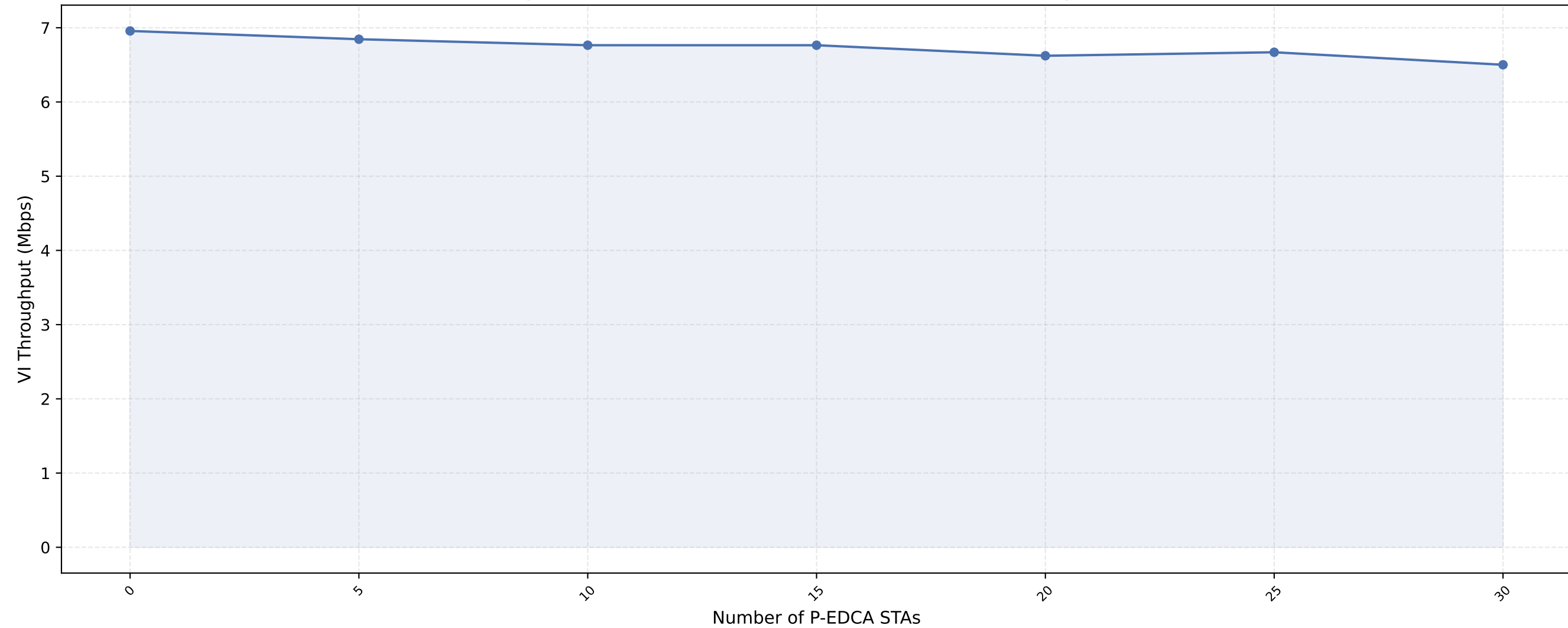
VI Throughput vs P-EDCA STAs — nSta=30, 1Mbps (avg of 10 runs)
