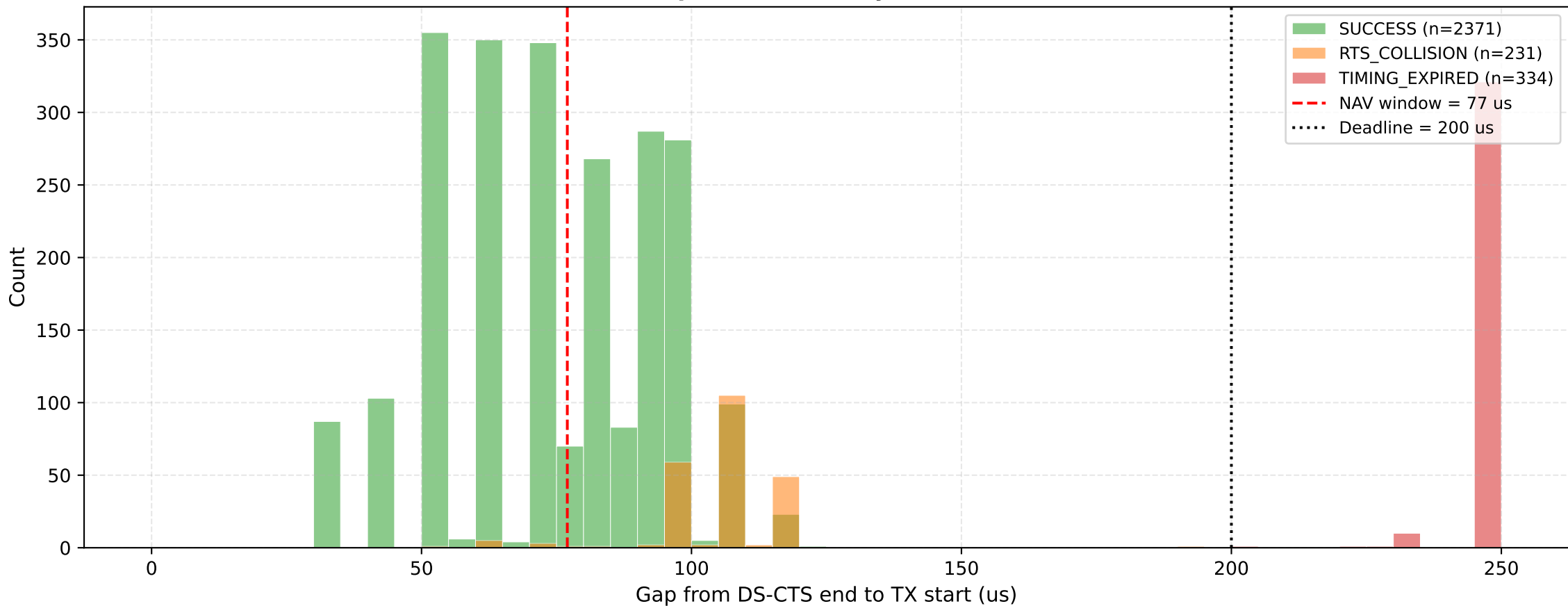
Gap Distribution by Outcome
