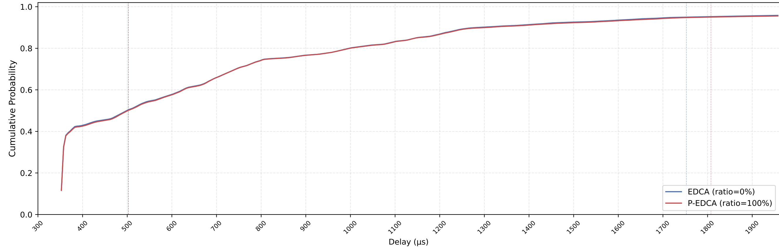
EDCA vs P-EDCA MAC Delay CDF — nSta=12, 1Mbps, avg of 10 runs
