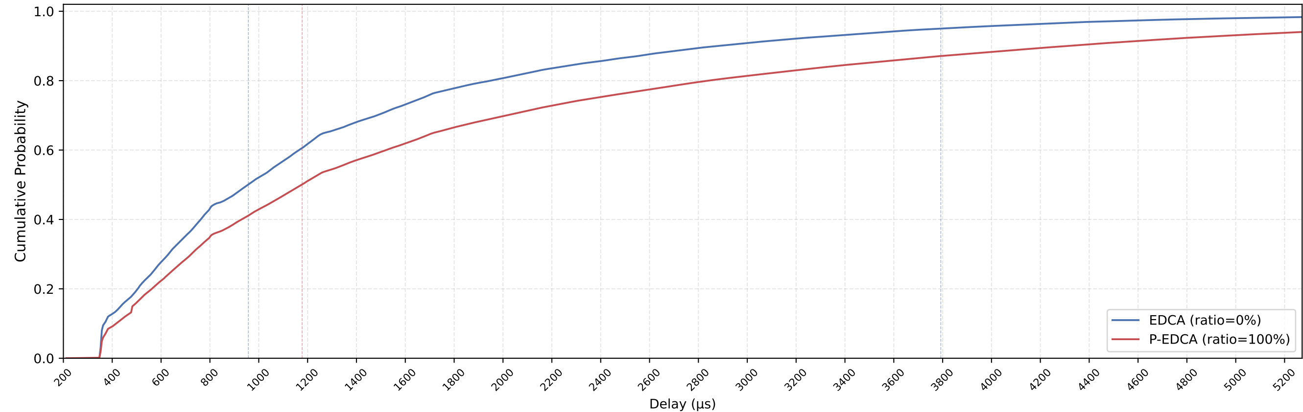
EDCA vs P-EDCA MAC Delay CDF — nSta=16, 1Mbps, avg of 10 runs
