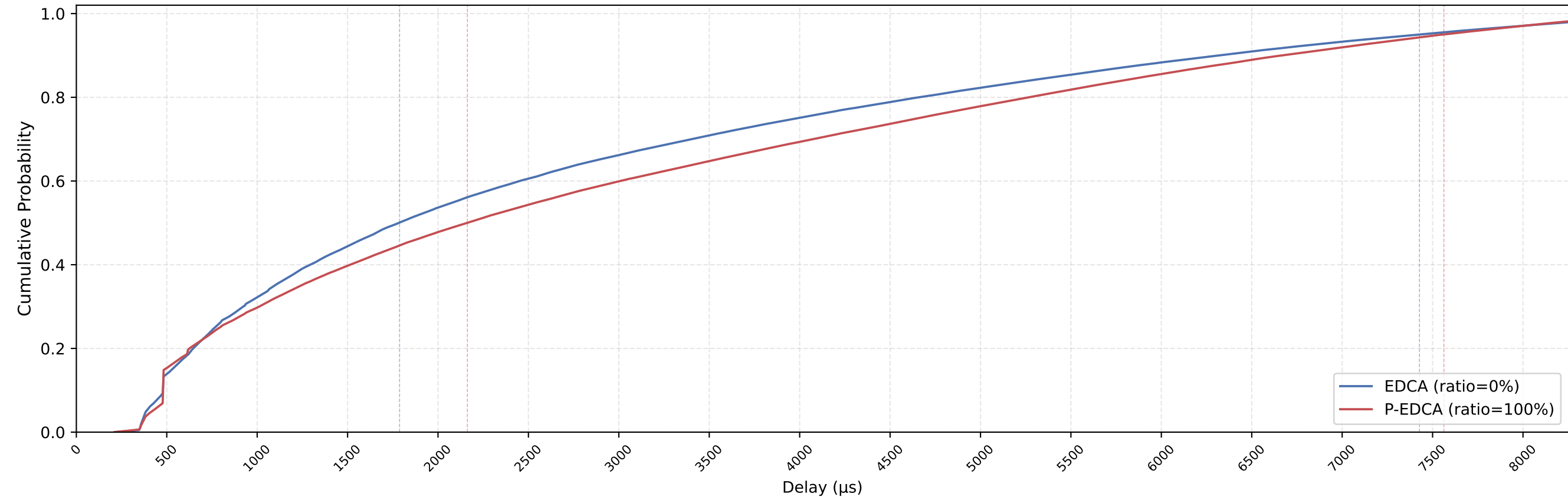
EDCA vs P-EDCA MAC Delay CDF — nSta=18, 1Mbps, avg of 10 runs
