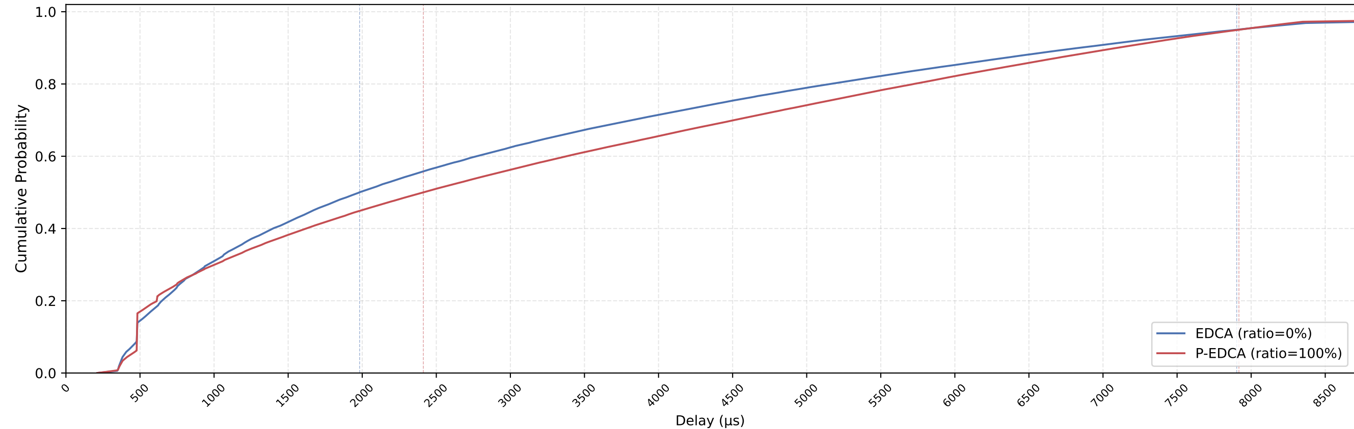
EDCA vs P-EDCA MAC Delay CDF — nSta=19, 1Mbps, avg of 10 runs
