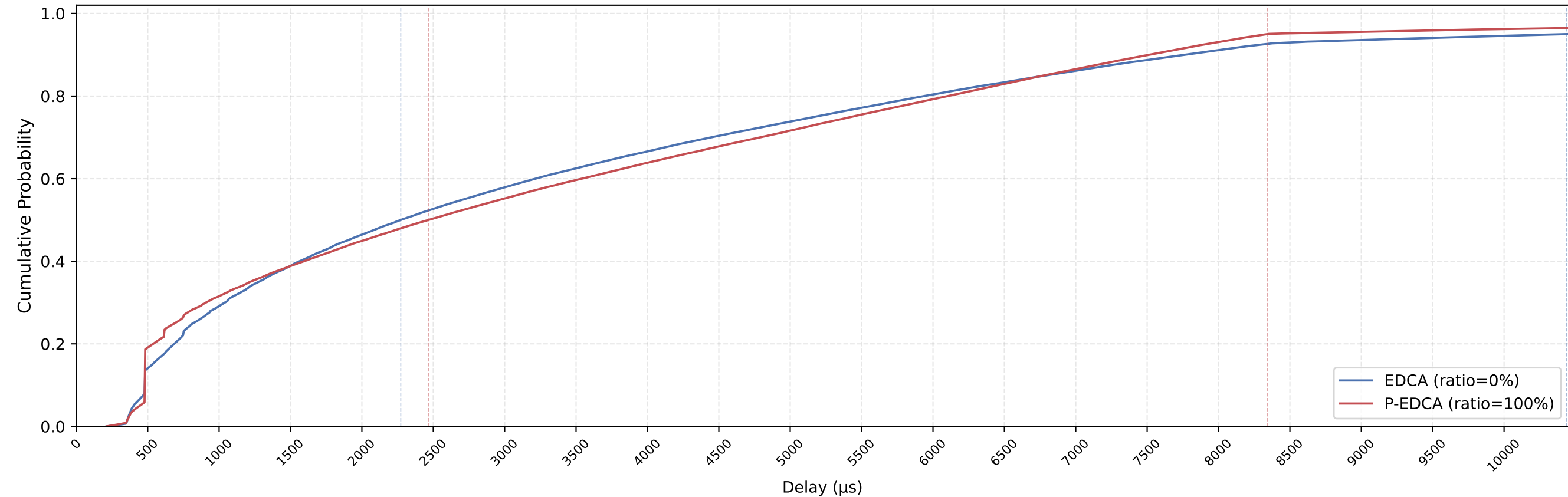
EDCA vs P-EDCA MAC Delay CDF — nSta=23, 1Mbps, avg of 10 runs
