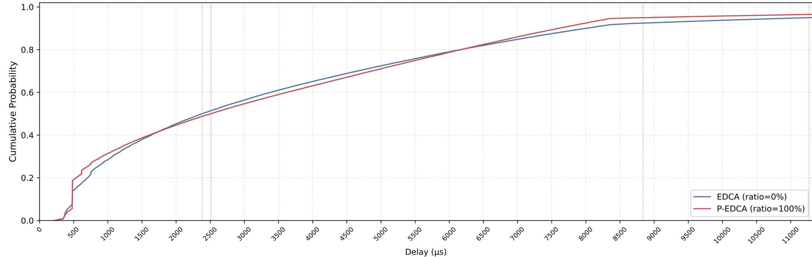
EDCA vs P-EDCA MAC Delay CDF — nSta=25, 1Mbps, avg of 10 runs
