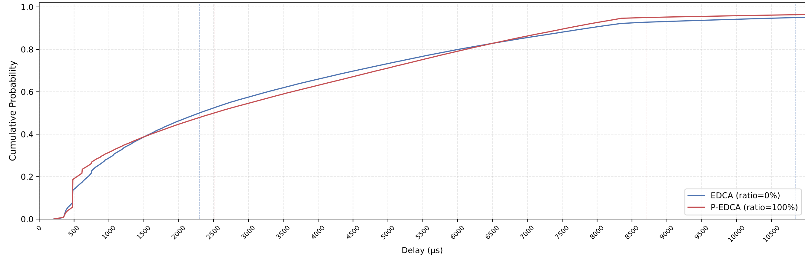
EDCA vs P-EDCA MAC Delay CDF — nSta=26, 1Mbps, avg of 10 runs
