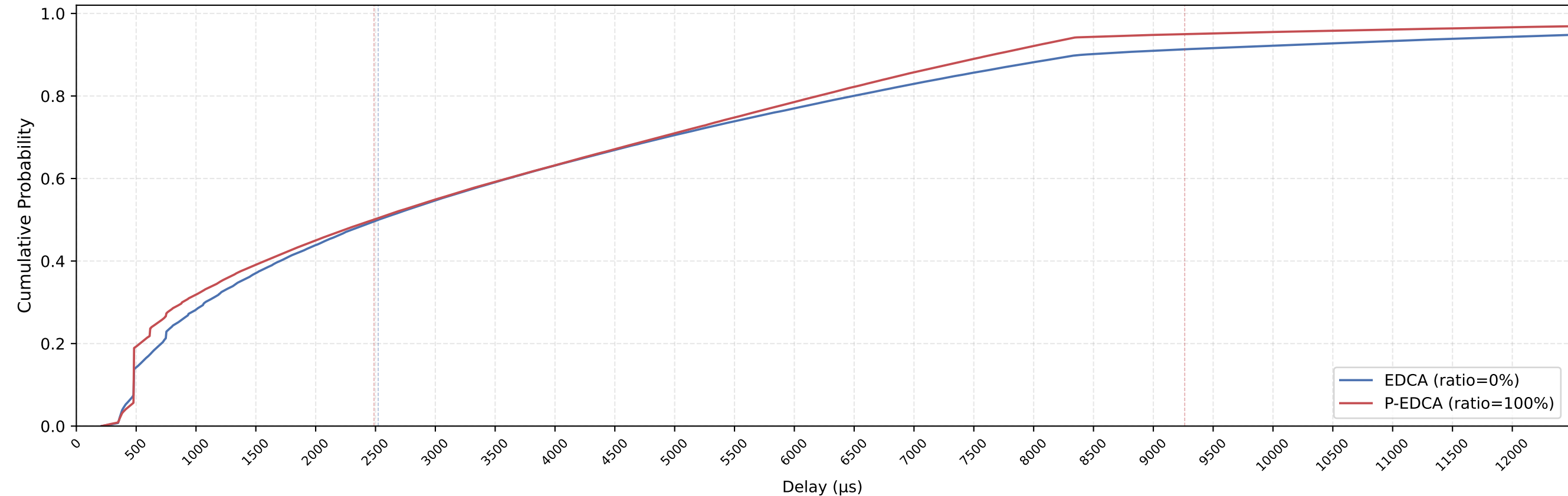
EDCA vs P-EDCA MAC Delay CDF — nSta=28, 1Mbps, avg of 10 runs
