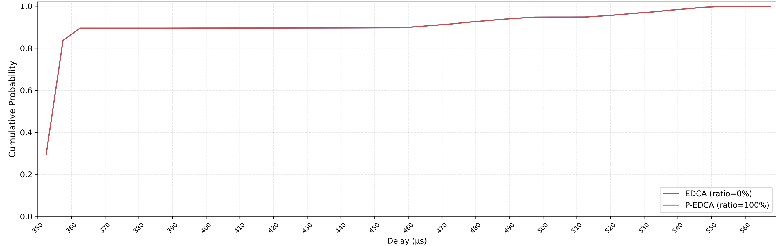
EDCA vs P-EDCA MAC Delay CDF — nSta=2, 1Mbps, avg of 10 runs
