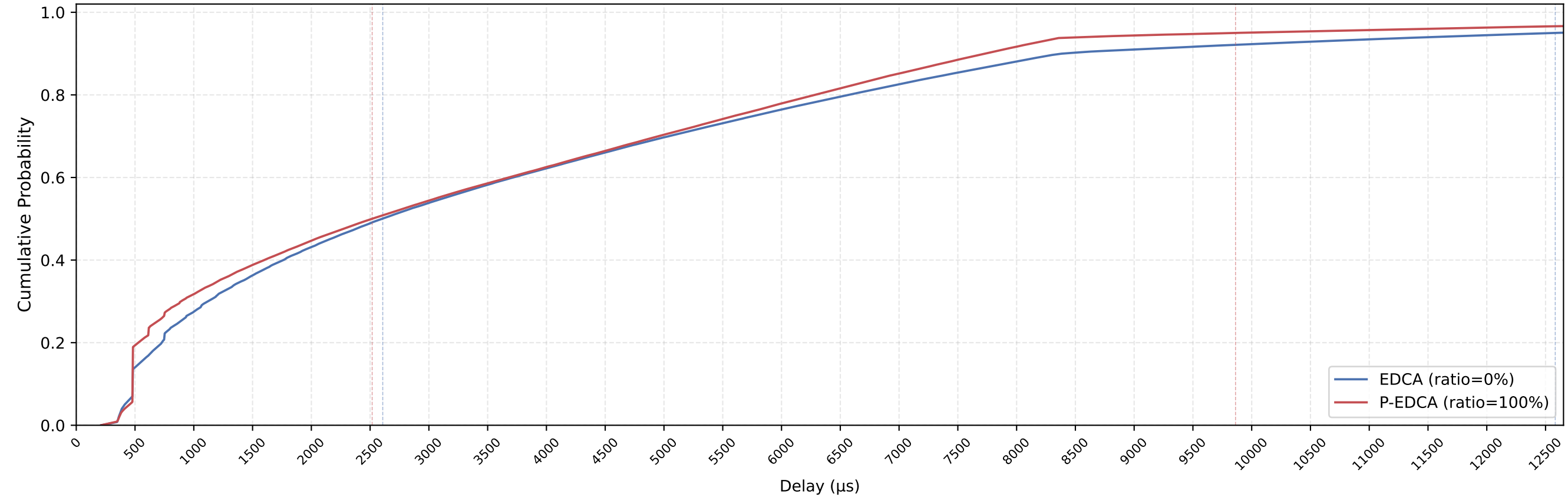
EDCA vs P-EDCA MAC Delay CDF — nSta=32, 1Mbps, avg of 10 runs
