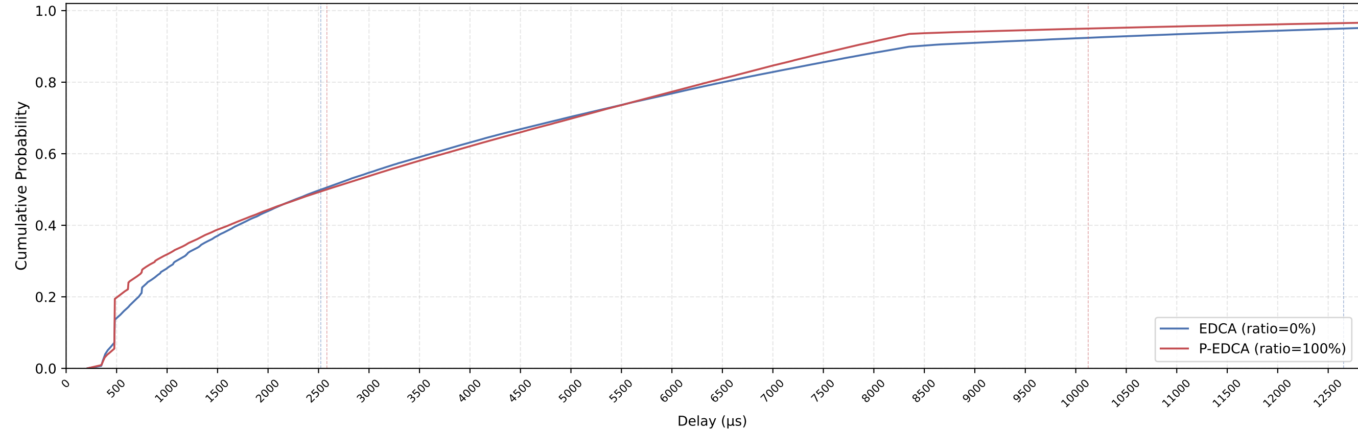
EDCA vs P-EDCA MAC Delay CDF — nSta=33, 1Mbps, avg of 10 runs
