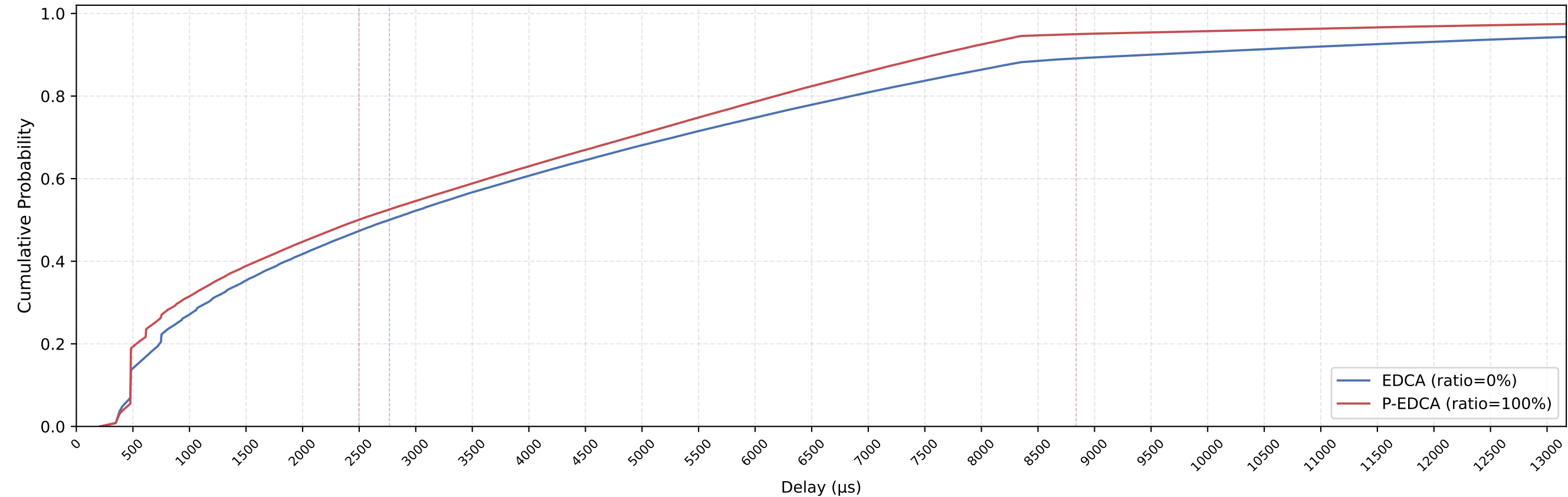
EDCA vs P-EDCA MAC Delay CDF — nSta=34, 1Mbps, avg of 10 runs
