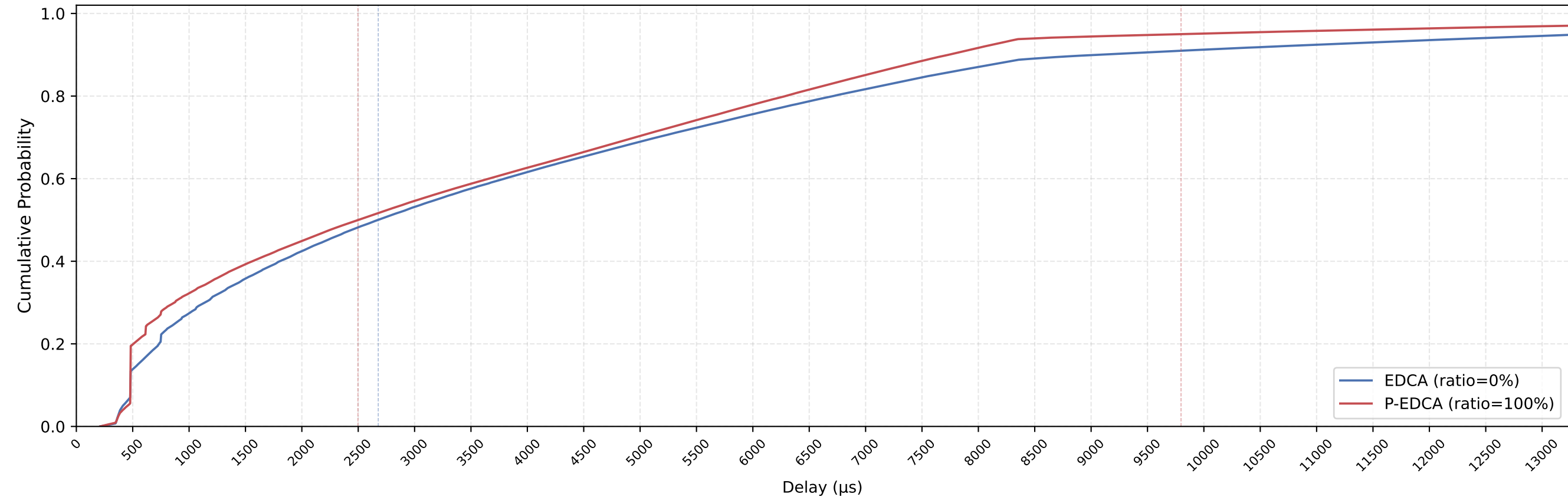
EDCA vs P-EDCA MAC Delay CDF — nSta=35, 1Mbps, avg of 10 runs
