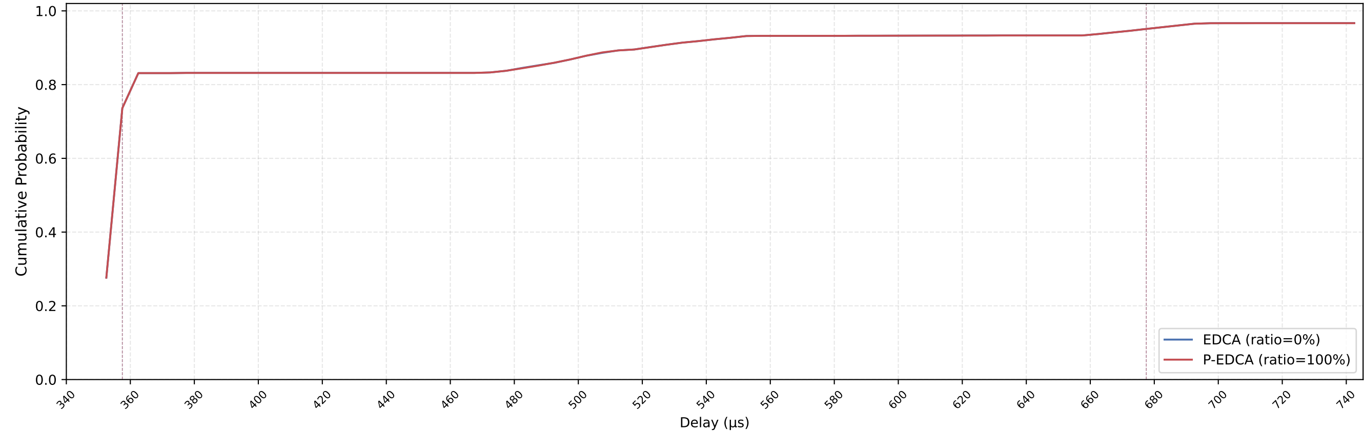
EDCA vs P-EDCA MAC Delay CDF — nSta=3, 1Mbps, avg of 10 runs
