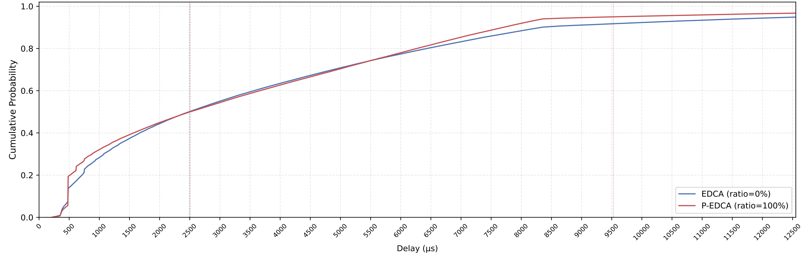
EDCA vs P-EDCA MAC Delay CDF — nSta=41, 1Mbps, avg of 10 runs
