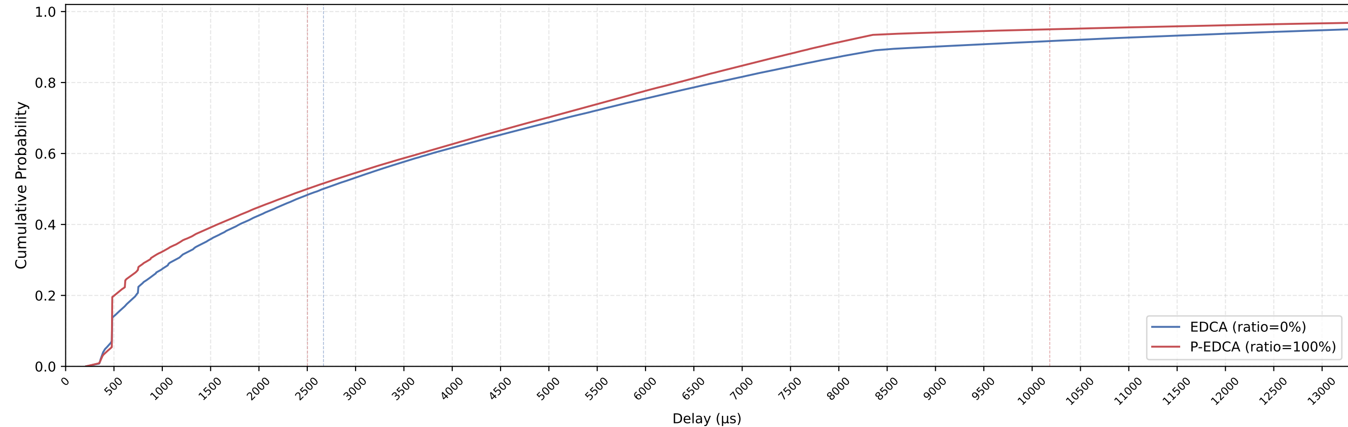
EDCA vs P-EDCA MAC Delay CDF — nSta=43, 1Mbps, avg of 10 runs
