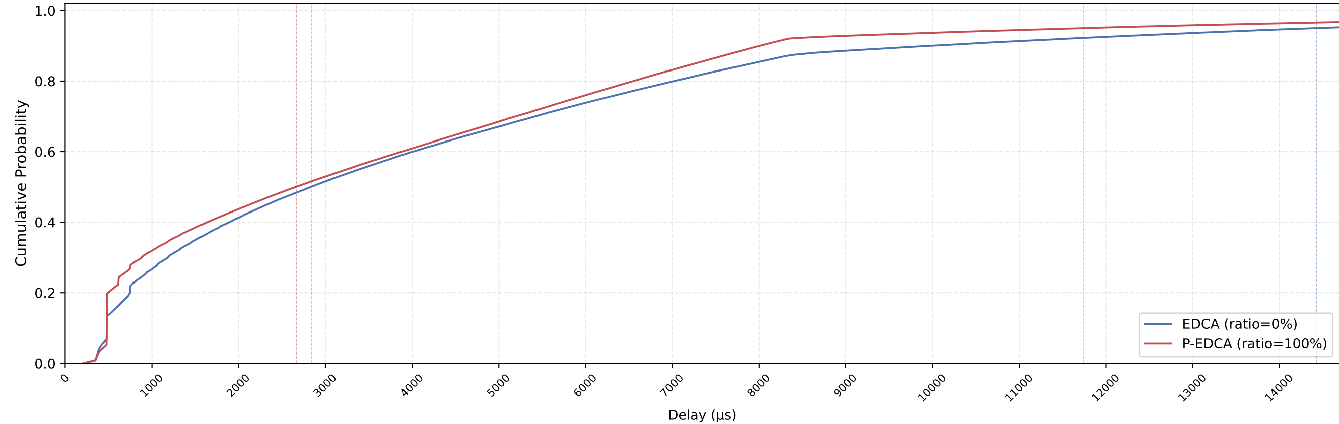
EDCA vs P-EDCA MAC Delay CDF — nSta=44, 1Mbps, avg of 10 runs
