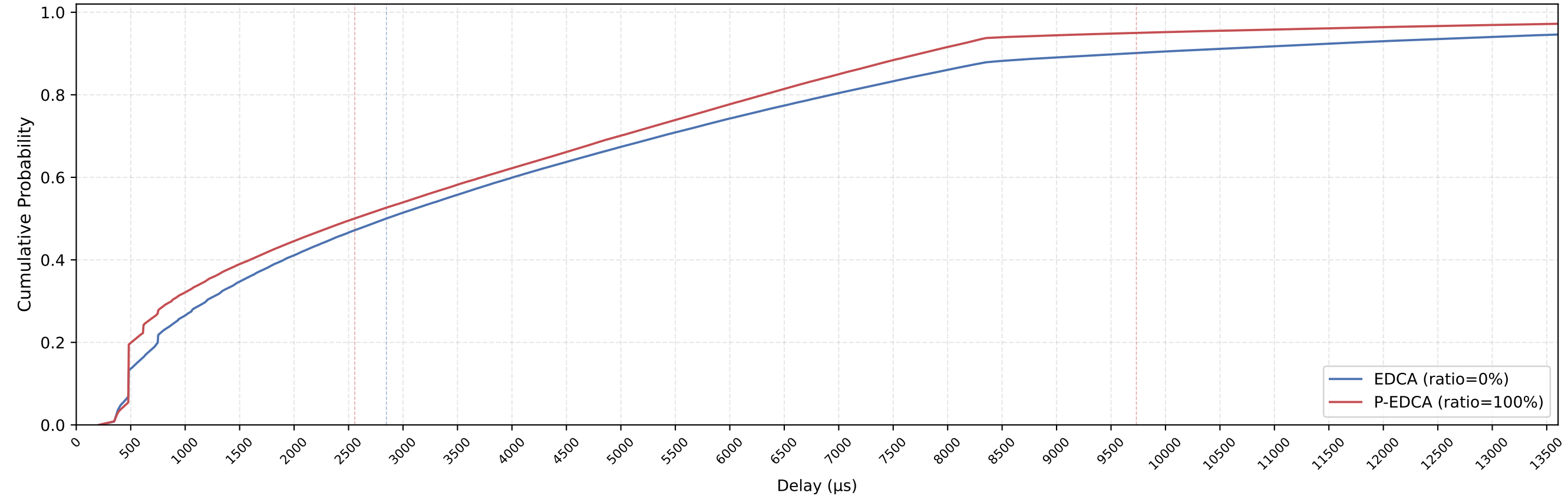
EDCA vs P-EDCA MAC Delay CDF — nSta=46, 1Mbps, avg of 10 runs
