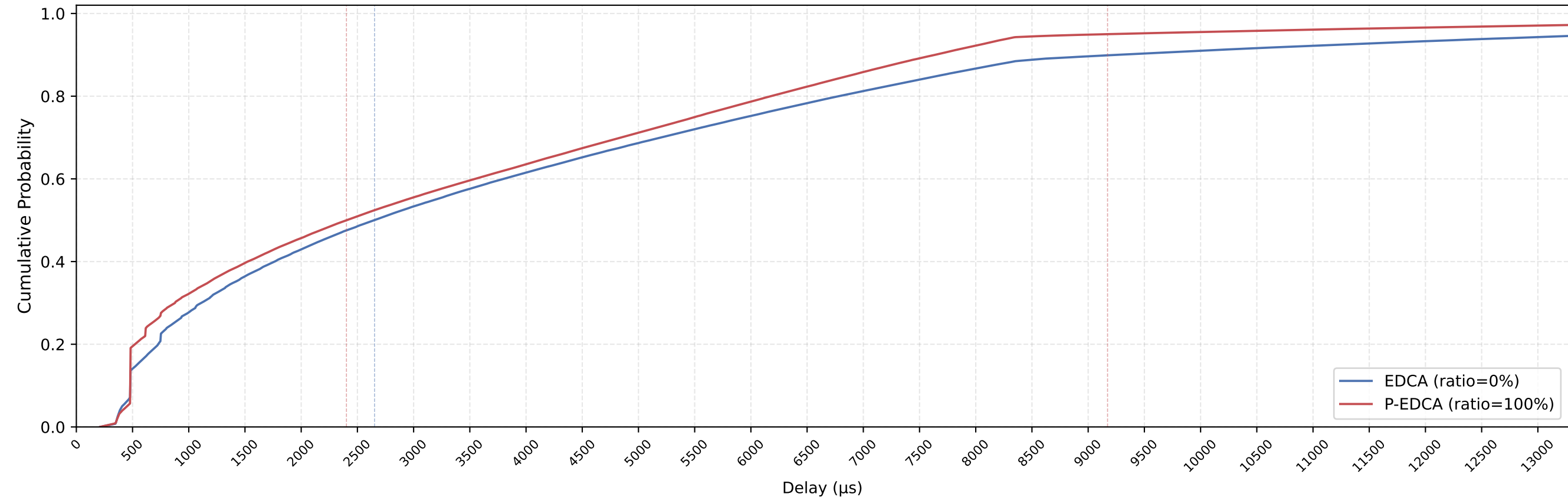
EDCA vs P-EDCA MAC Delay CDF — nSta=47, 1Mbps, avg of 10 runs
