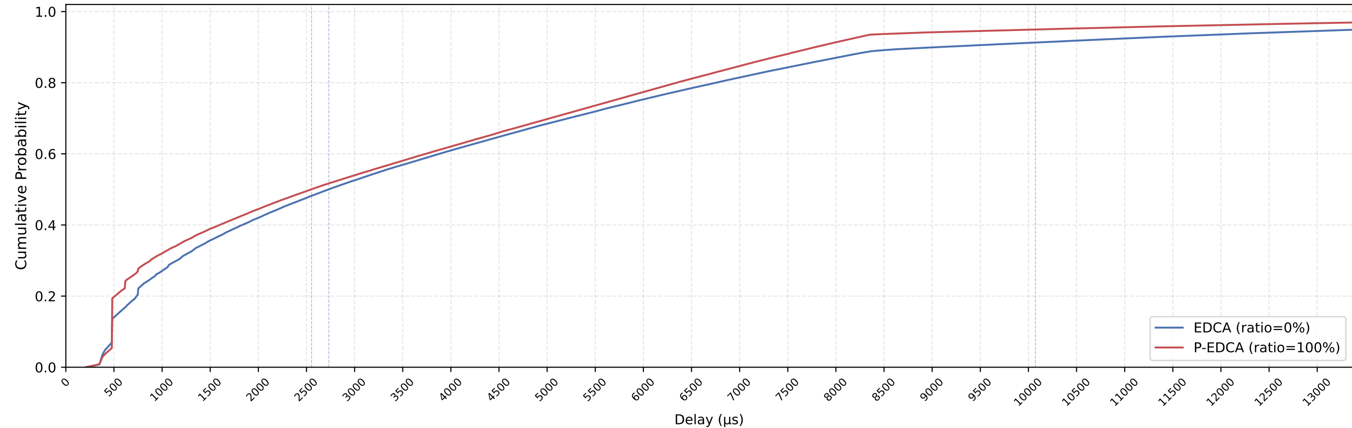
EDCA vs P-EDCA MAC Delay CDF — nSta=48, 1Mbps, avg of 10 runs
