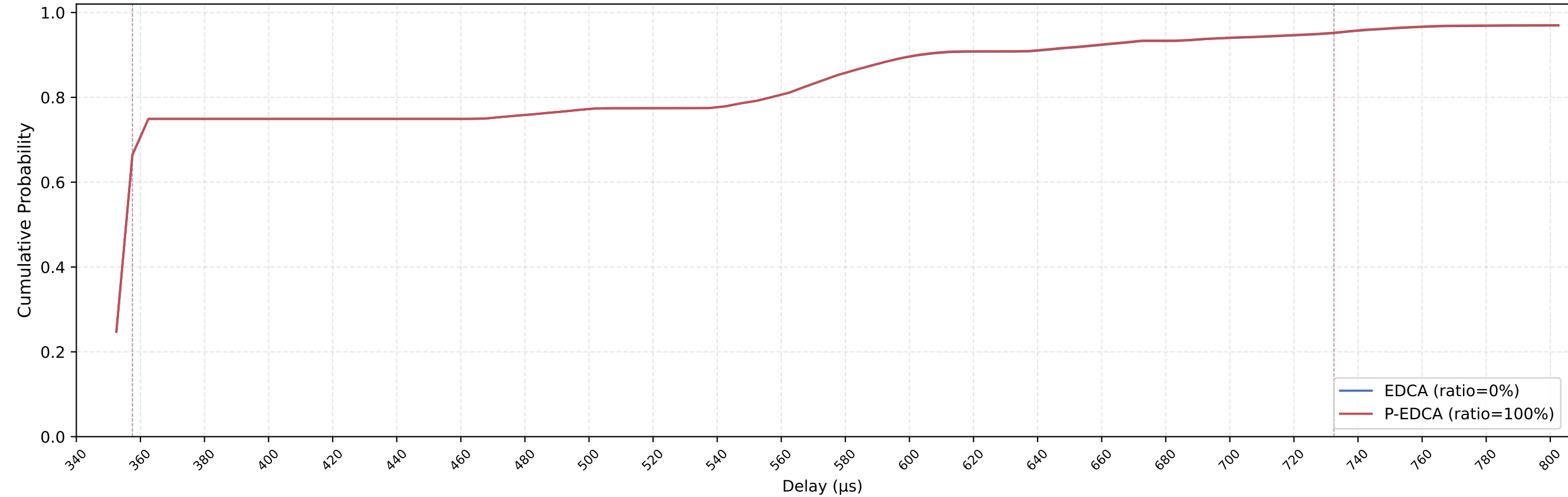
EDCA vs P-EDCA MAC Delay CDF — nSta=4, 1Mbps, avg of 10 runs
