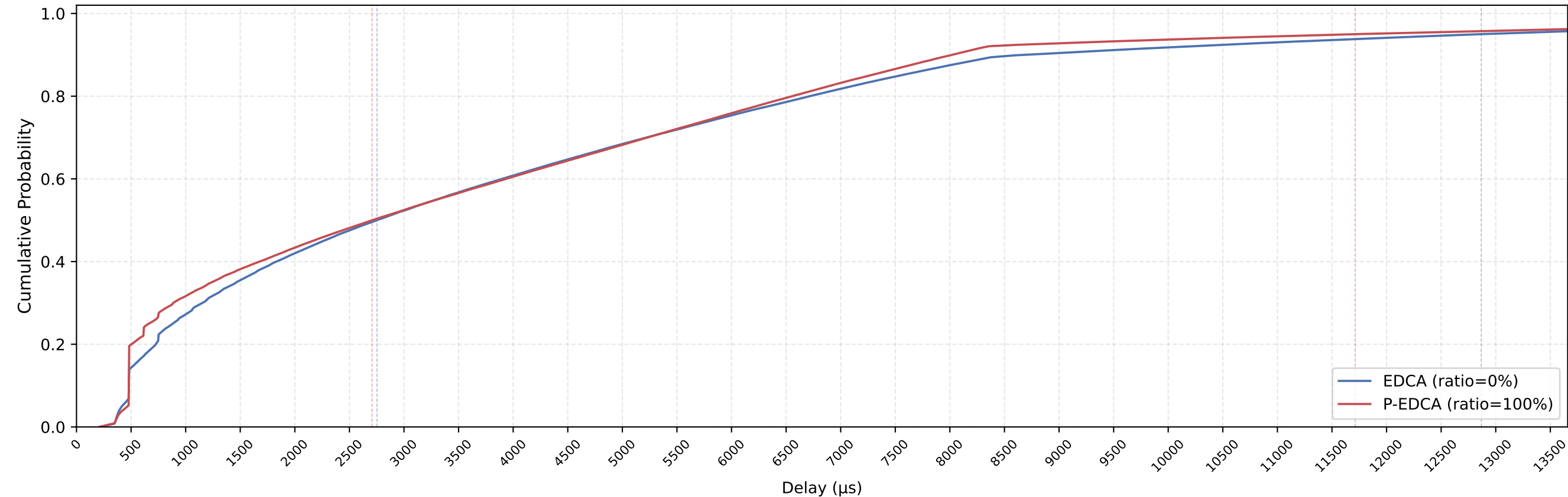
EDCA vs P-EDCA MAC Delay CDF — nSta=50, 1Mbps, avg of 10 runs
