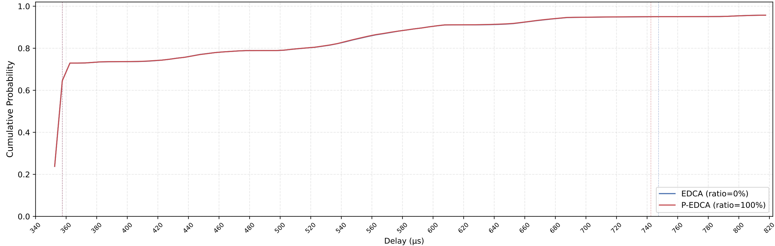
EDCA vs P-EDCA MAC Delay CDF — nSta=6, 1Mbps, avg of 10 runs
