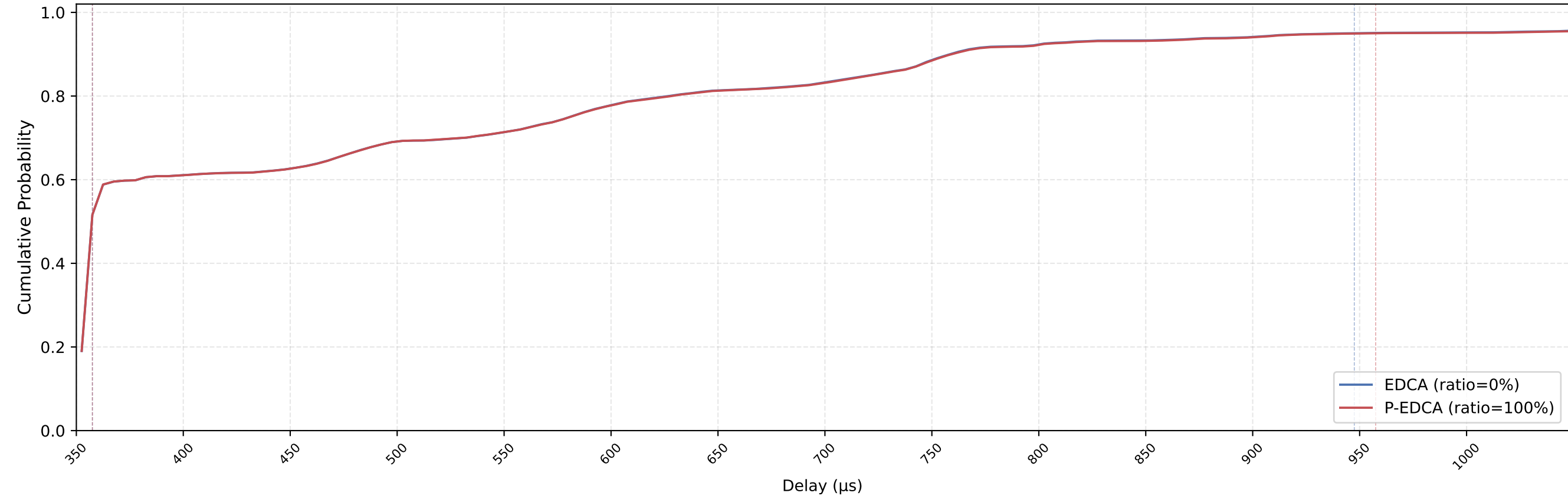
EDCA vs P-EDCA MAC Delay CDF — nSta=8, 1Mbps, avg of 10 runs
