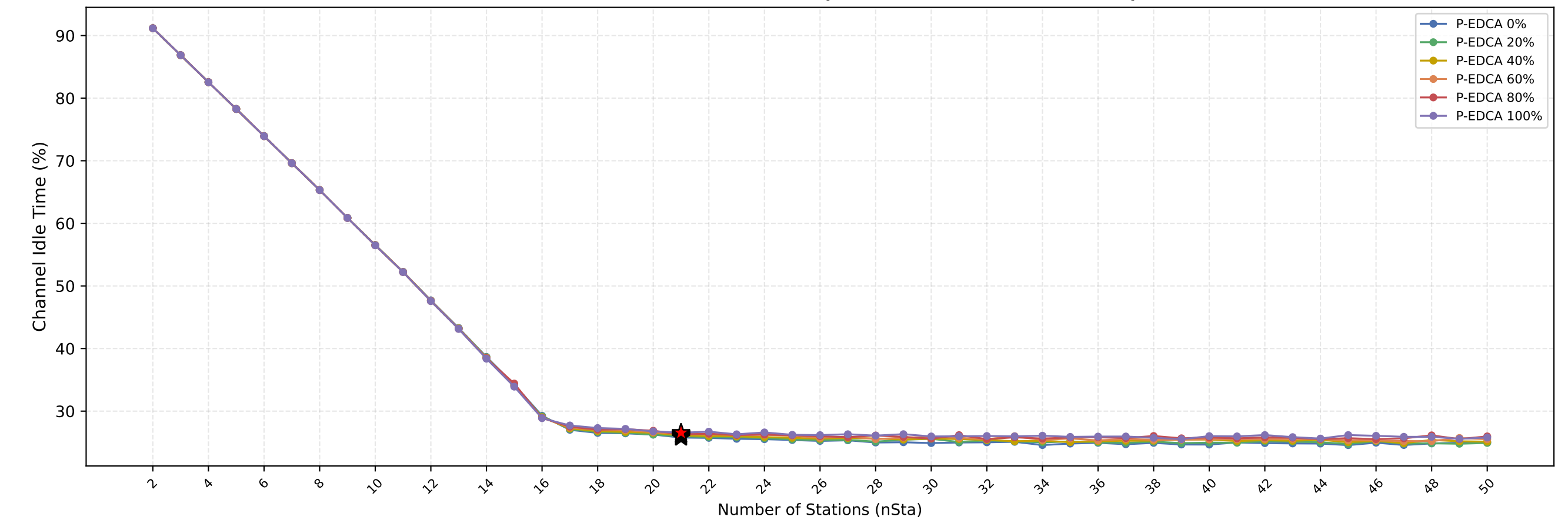
Channel Idle Time vs nSta — (Red Star = Current nSta=21)
