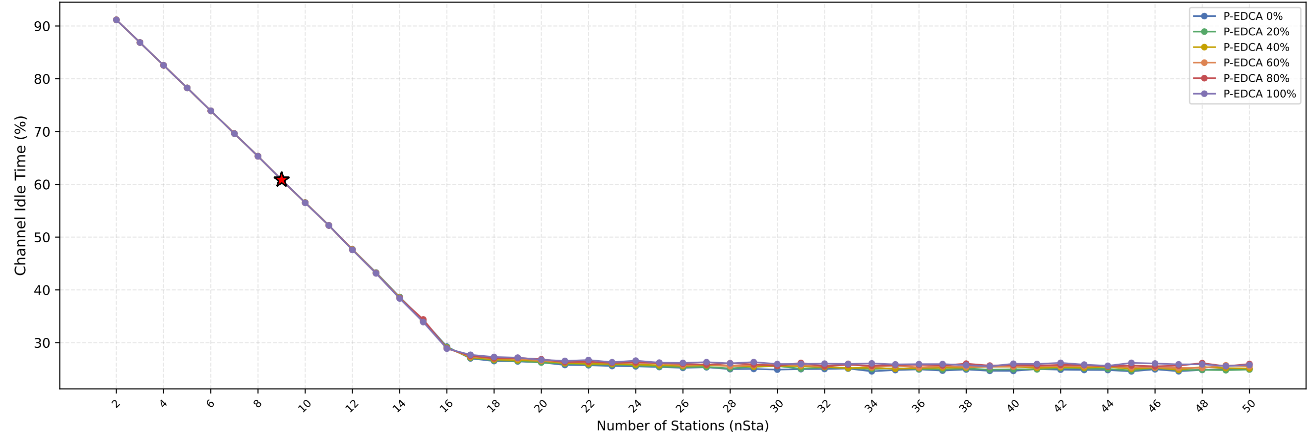
Channel Idle Time vs nSta — (Red Star = Current nSta=9)
