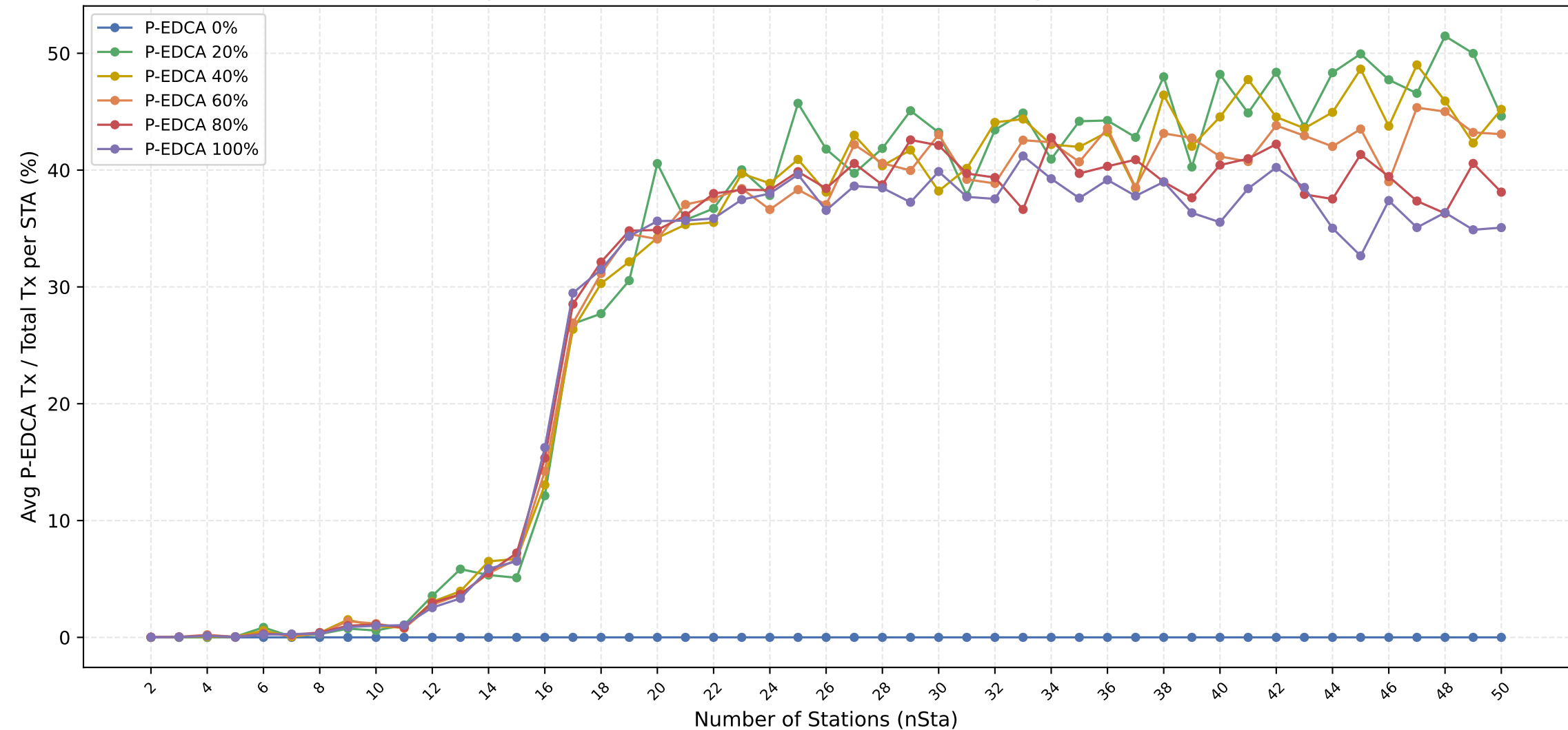
Avg P-EDCA Tx Ratio vs nSta — 1Mbps (avg of 10 runs)
