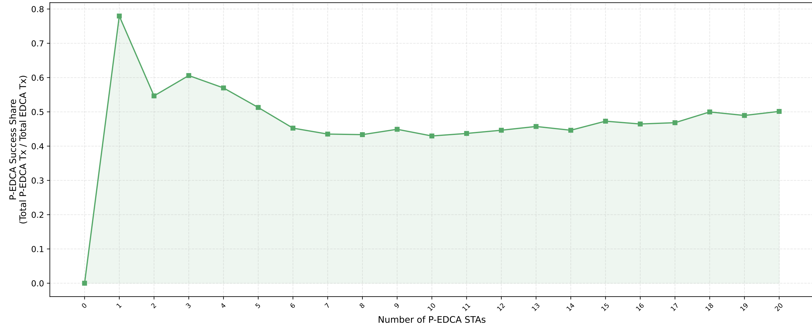
P-EDCA Tx / Total EDCA Tx — nSta=20, 1Mbps (avg of 10 runs)
