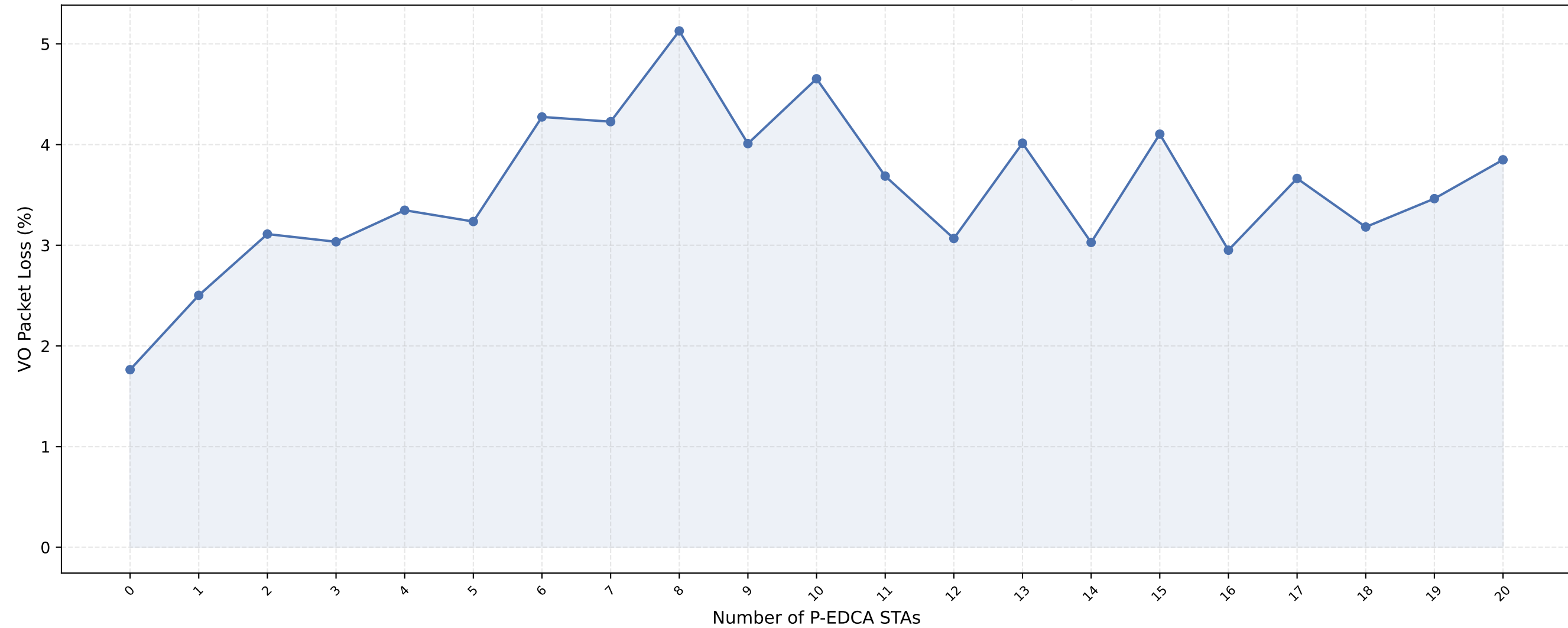
VO Packet Loss vs P-EDCA STAs — nSta=20, 1Mbps (avg of 10 runs)
