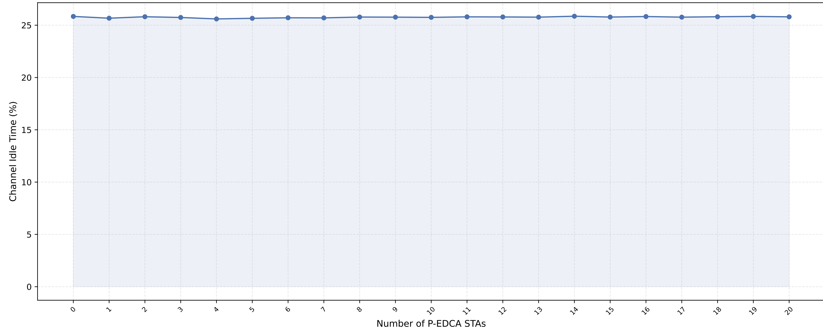
Channel Idle Time vs P-EDCA STAs — nSta=20, 1Mbps (avg of 10 runs)
