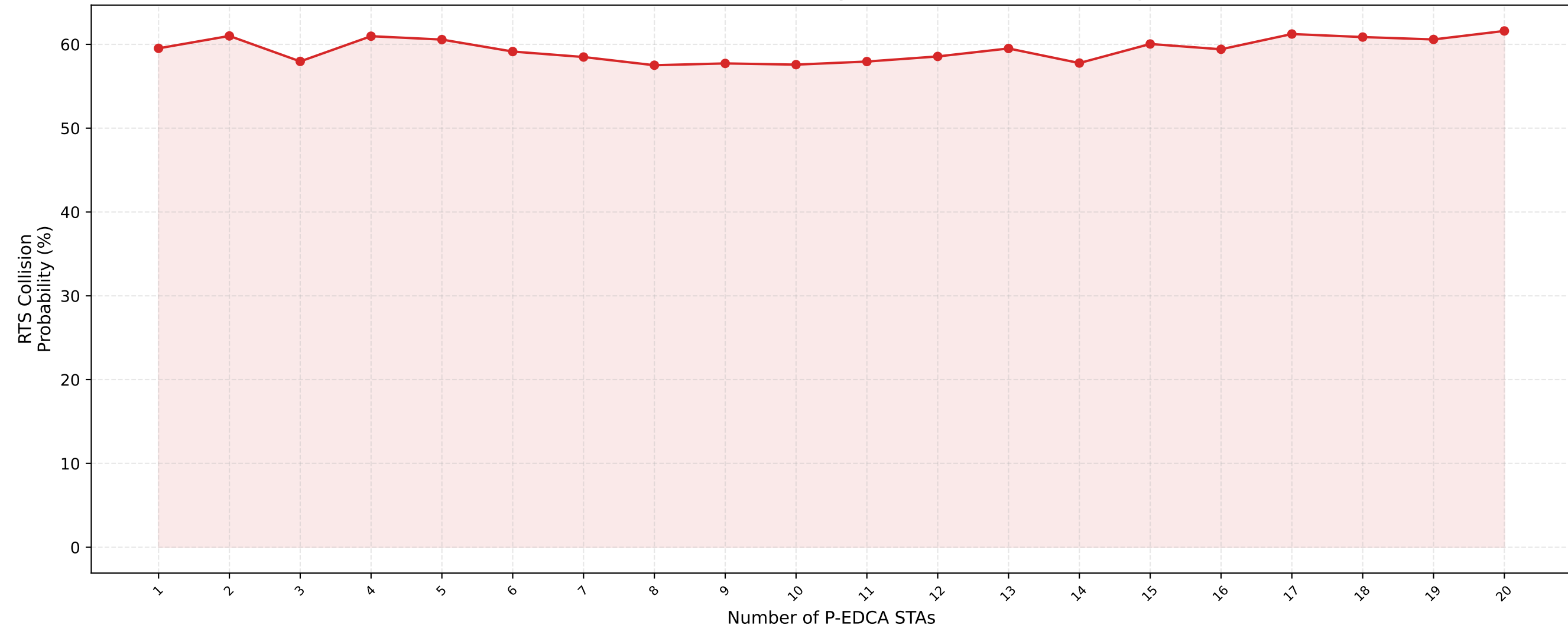
[Stat 6] P-EDCA RTS Collision Probability — nSta=20, 1Mbps (avg of 10 runs)
